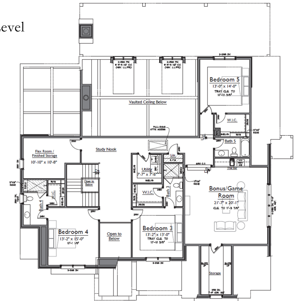
1 UPPER LEVEL FLOOR PLAN 1/8" = 1'-0"
