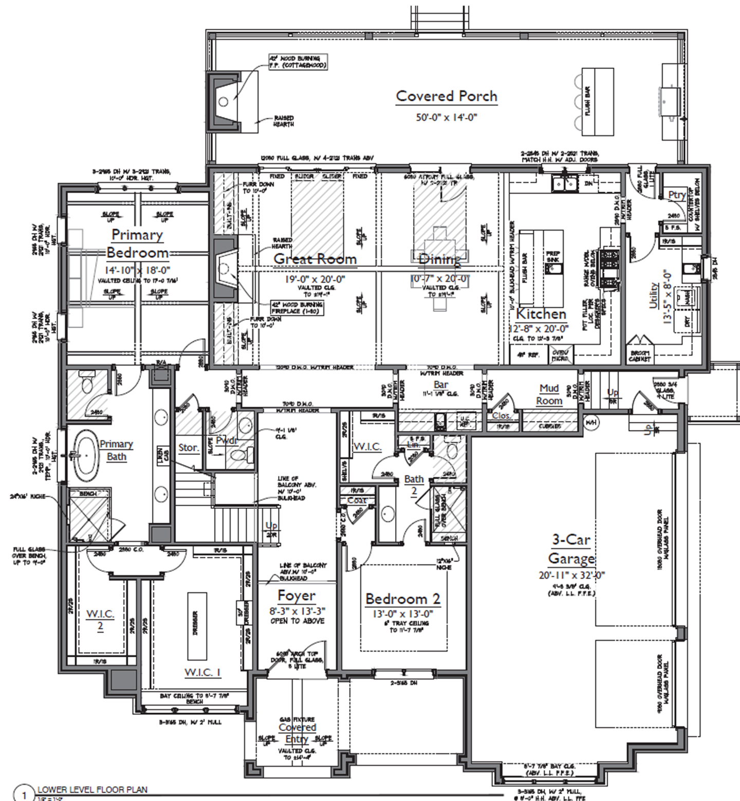
Main Level
