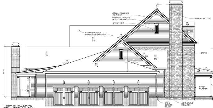
LEFT ELEVATION
