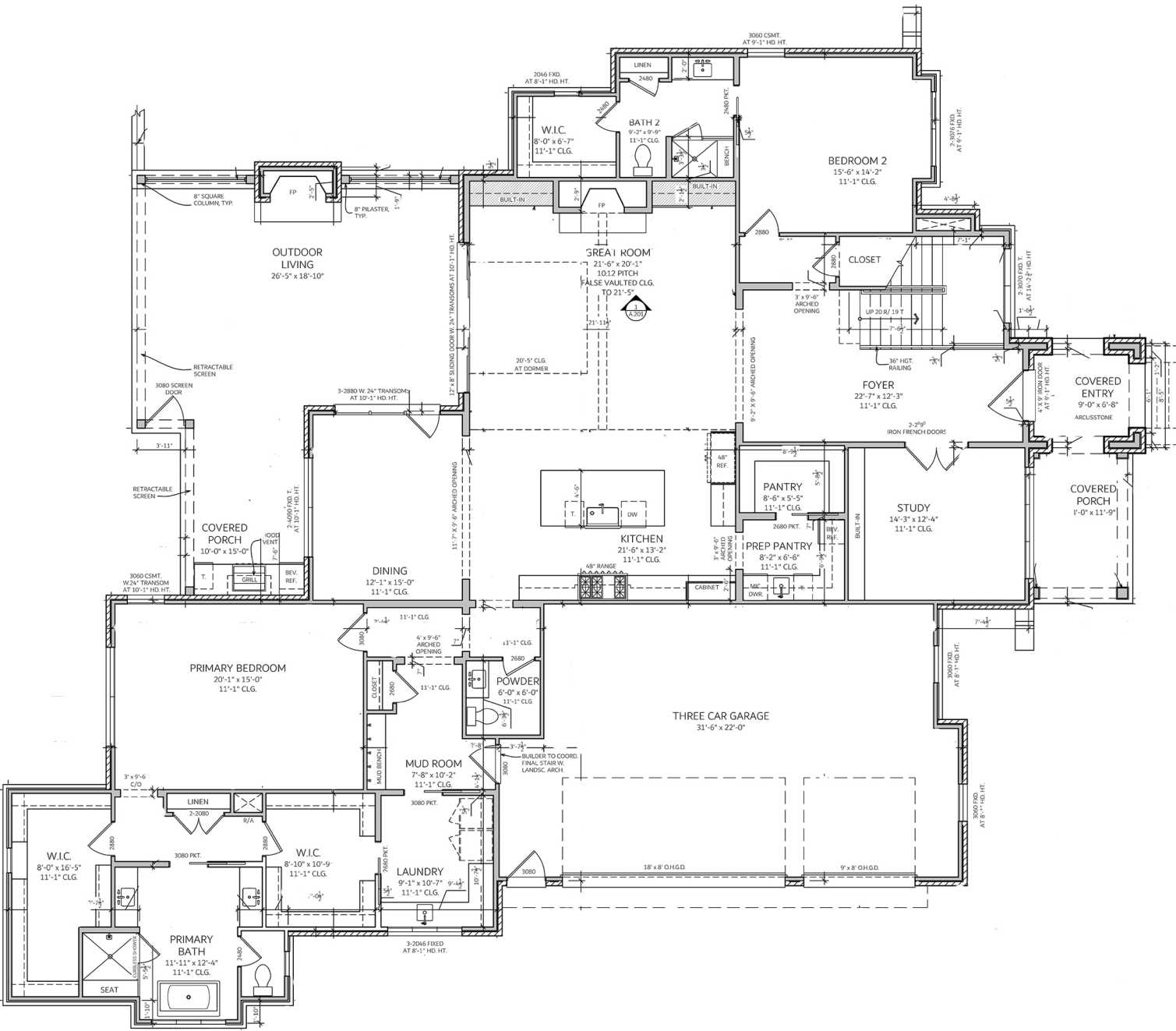
Main Level
