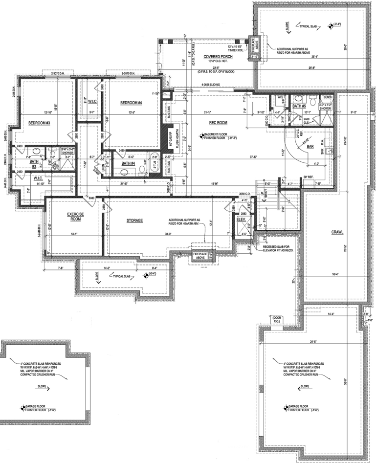
Lower Level
