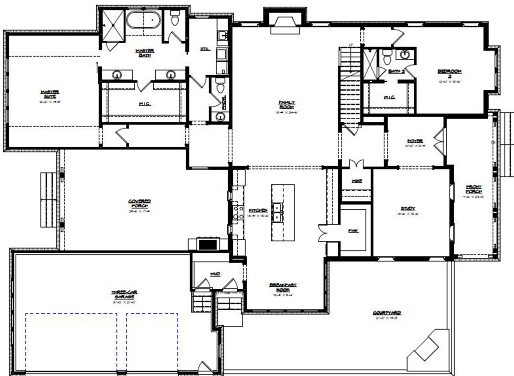
FIRST FLOOR PLAN 1/4" = 1'-0"
