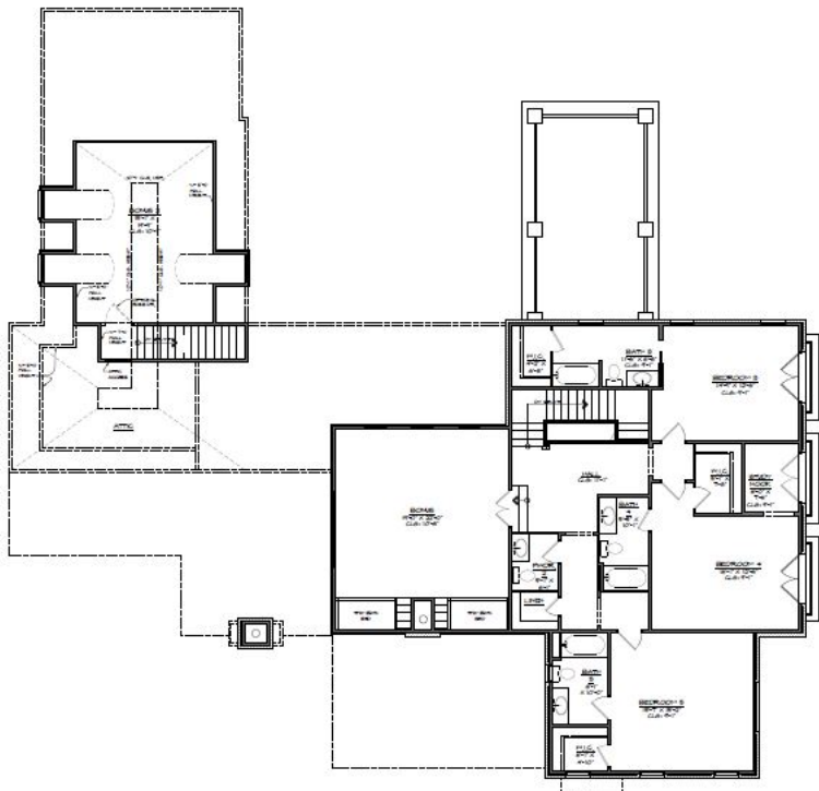
UPPER LEVEL LIGHTING SCHEMATIC SCALE 1/4" = 1'-0"
